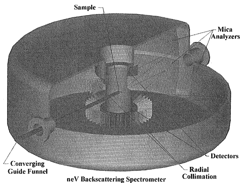
Figure 1 – The layout of the neV-backscattering guide system at the LWTS at SNS.
