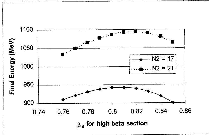
Figure 2. Final beam energy vs. the high beta cryomodule \beta_g , for 11 medium beta cryo-modules with \beta_g = 0.61 , 17 and 21 high beta cryo modules, and a lower peak surface field of 25 MV/m.
