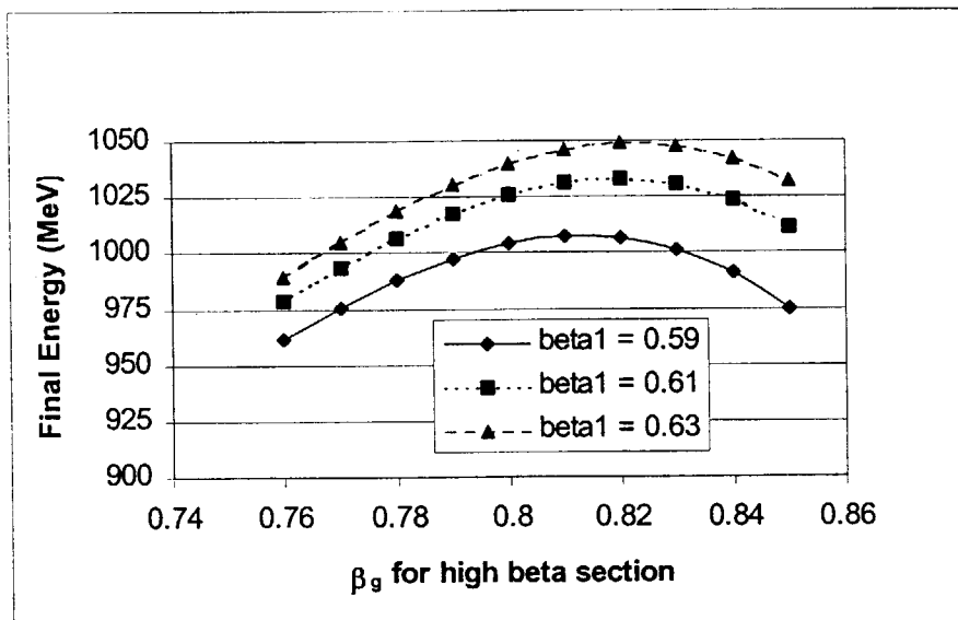
Figure 1. Final beam energy vs. the high beta cryomodule \beta_g , for three different medium beta cryomodule \beta_g values. The reference peak surface field of 27.5 MV/m is used here, with 11 medium beta cryo-modules and 17 high beta cryo-modules. .
