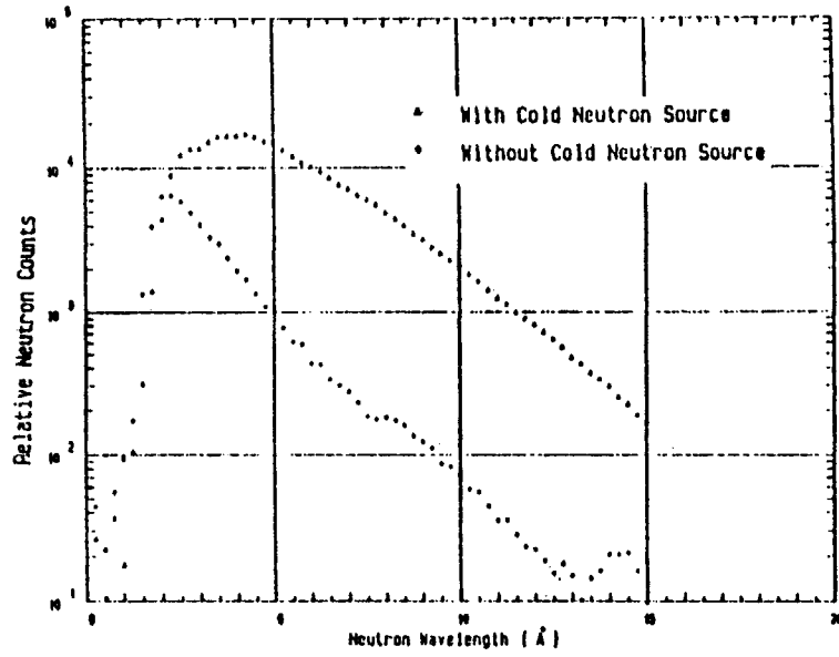
Fig.1 Neutron Spectra Measured at the Guide Exit
