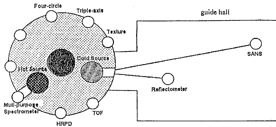
Fig. 2 layout of neutron scattering facilities at CARR
