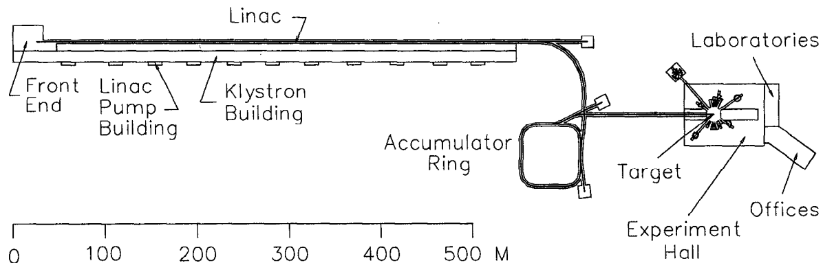
Figure 1. Proposed layout of the SNS facility.
