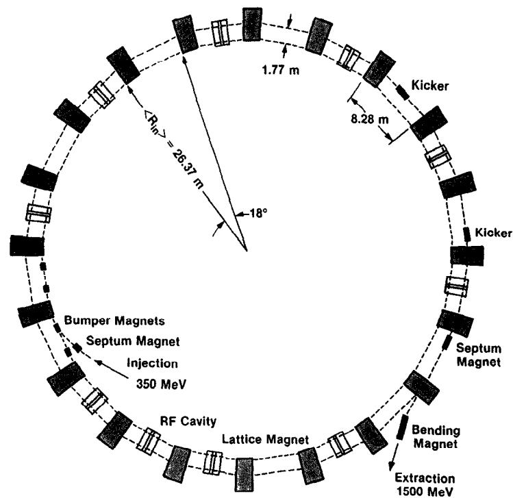
Fig. 2 Layout of radial-sector FFAG for ASPUN.
