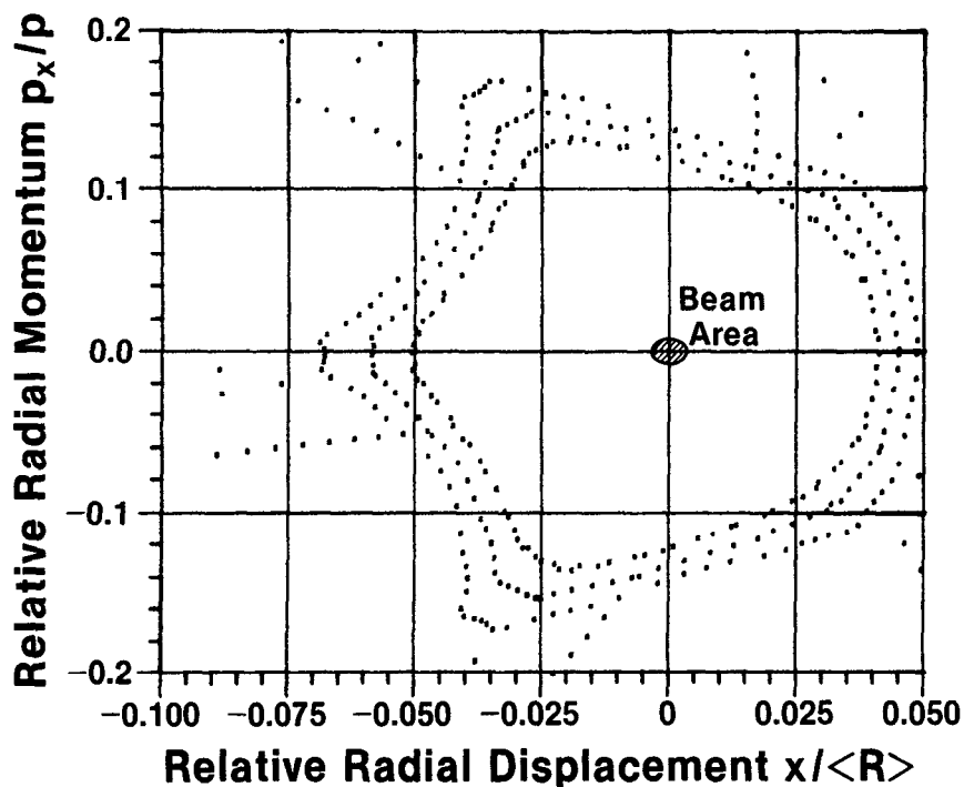
Fig. 6 Limits of beam stability in horizontal plane due to magnet nonlinearities with the 650\text{-}\pi\text{mmmr} beam emittance shown in shaded area.
