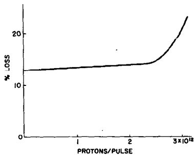
Fig. 1. Total beam losses between injection and extraction. The increase in losses at high intensity is primarily due to capture losses.
