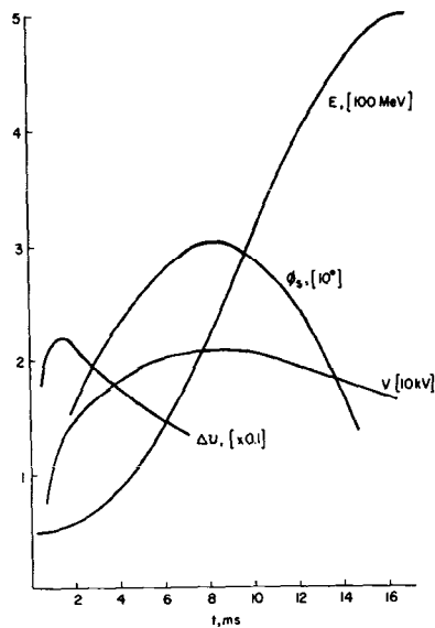
Fig. 2. Present operating conditions of the RCS.
