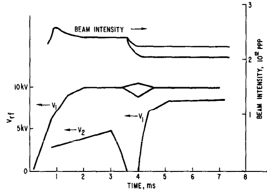
Fig. 8. Beam intensity during transition from harmonic to fundamental operation. The range of beam losses due to changes in the fundamental voltage is shown.
