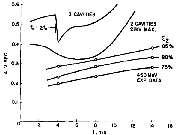
Fig. 4. Phase space acceptance and measured longitudinal emittance as a function of time, for 2 and 3 cavities.
