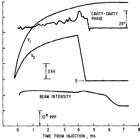
Fig. 6. Typical harmonic operating conditions.
