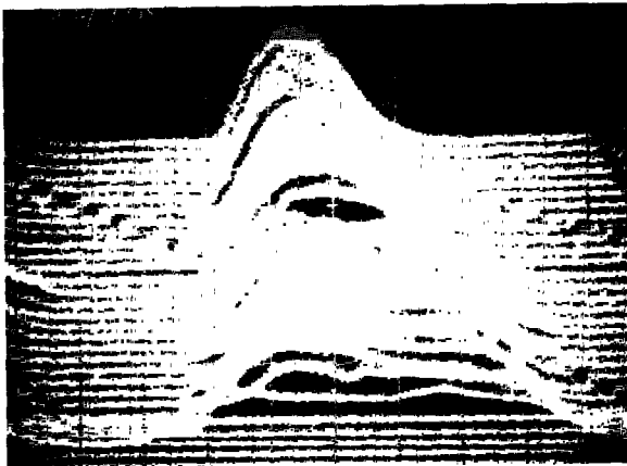
Fig. 7. Mountain range display of fundamental and harmonic bunch structure and the transition to the fundamental. Horizontal scale - 50 ns/division.
