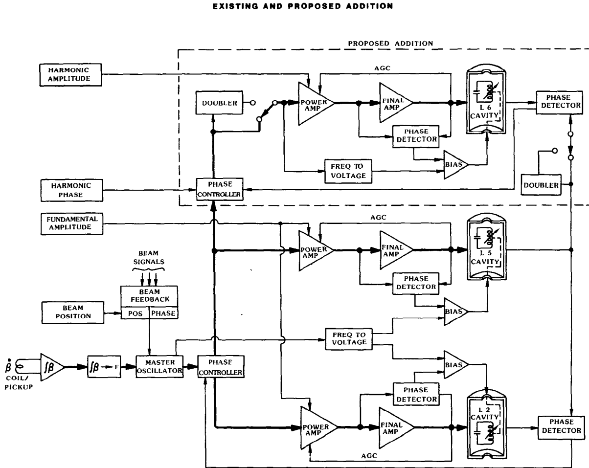
Fig. 5. Block diagram of the existing and proposed accelerating systems.
