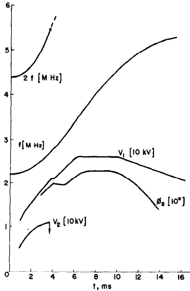
Fig. 3. Voltage and frequency programs for the two harmonics.
